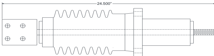
ENTRANCE BUSHING 600 AMPS 34.5 kV 200 B.I.L
