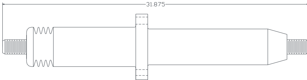
ENTRANCE BUSHING 1200 AMPS
